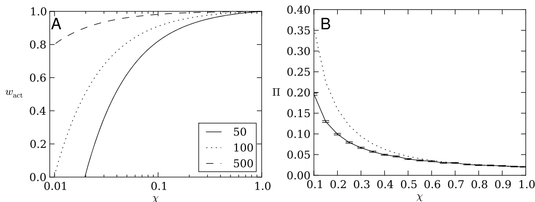
Figure 1 | (A) Fitness ( w_{act} ) as a function of strategy choice \chi and population size according to Gillespie's model Equation (6). Fitness differences between strategies with different \chi are far more pronounced in smaller populations. Larger population sizes effectively buffer risky strategies against immediate extinction when the risky strategy does not pay off. See legend for population sizes. We note that the x-axis is log scale. (B) Fixation probability ( \Pi ) of a perfectly risk-sensitive strategy ( \chi = 1 ) within a uniform background of strategies with choice \chi , as a function of \chi (solid line). Fixation probabilities were estimated from 100,000 repeated runs, each seeded with a single invading strategy with \chi = 1 in a background population of N = 50 resident strategies with strategy \chi . The dashed line is Kimura's fixation probability \Pi(s) = (1 - e^{-2s}) / (1 - e^{-2Ns}) (see, e.g., Ref. 55), where s is the fitness advantage of the invading strategy calculated using Equation (6). Error bars are two standard errors.
