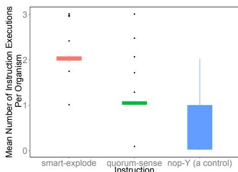
Figure 4: The average instruction executions for smart-explode, quorum-sense and a neutral instruction per organism in the population. The smart-explode instruction was used 1.95 more per organism than the neutral instruction ( nop-Y ) in the last 100 updates. The quorum-sense instruction was used 0.99 more per organism than the neutral instruction ( nop-Y ) in the last 100 updates (95% CI for difference between smart-explode and neutral instruction is 1.92 to 1.97 executions per organism, Wilcoxon rank sum test p < 0.0001 ; 95% CI difference quorum-sense instruction executions and neutral instruction is 0.96 to 1.00 executions per organism, Wilcoxon rank sum test p < 0.0001 , error bars represent 95% confidence intervals). Both quorum sensing and suicidal altruism are under positive selection in this environment.
